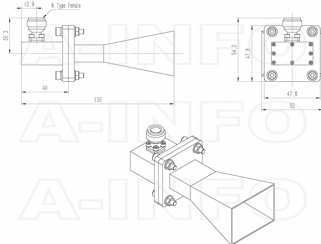
N-Female Output (P/N: LB-112-10-C-NF)
