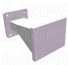
LB-112-10-ASPO Standard Gain Horn Antenna 7.05-10GHz 10dB Gain Rectangular Waveguide Interface
